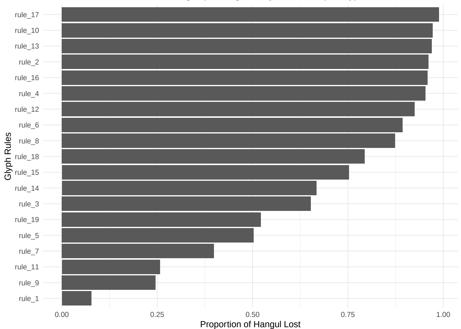
Effect of Rule Removal on Hangul (Unweighted by Word Frequency)
